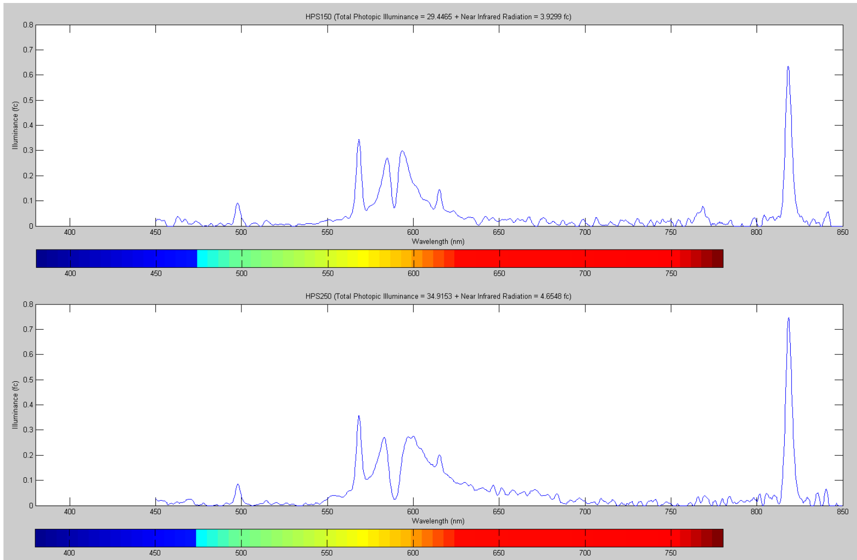
Figure 39: Light Spectrum (including near Infrared) for a) HPS 150 and b) HPS 250 at Floor Level (0 Feet) at the Center of Light
