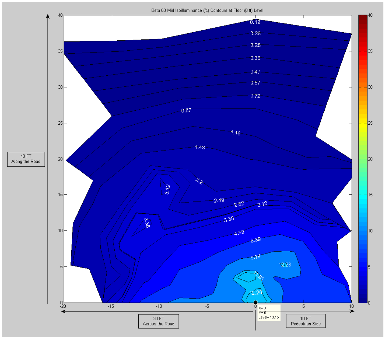
Figure 7: Contour Plot of Isoilluminance (fc) for Beta 60 LED Mid Driver Setting at the Floor (0 Feet) Level on Measurement Grid
