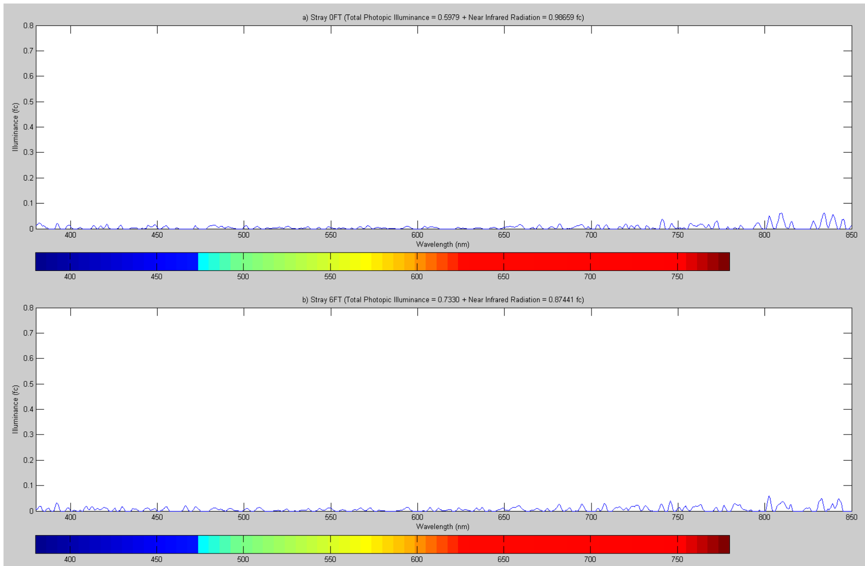
Figure 38: Stray Light Spectrum (including near Infrared) at Floor Level (0 Feet) at the Center of Light
