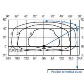
Isofootcandle plot of 6000K, 60 LED Type III Medium streetlight luminaire with backlight control at 25' A.F.G. Luminaire with 5,123 initial delivered lumens operating at 525mA. Initial FC at grade.
