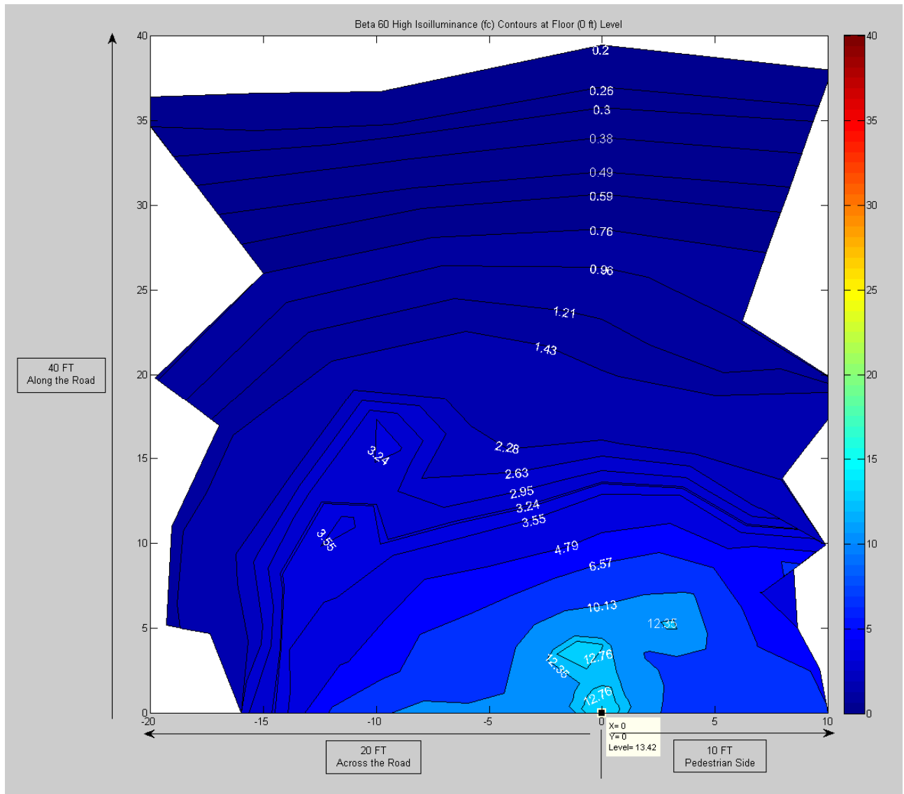
Figure 8: Contour Plot of Isoilluminance (fc) for Beta 60 LED High Driver Setting at the Floor (0 Feet) Level on Measurement Grid
