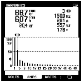
Voltage, current, and power harmonics Up to 51st harmonic Total harmonic distortion (THD) Phase angle of individual harmonics
