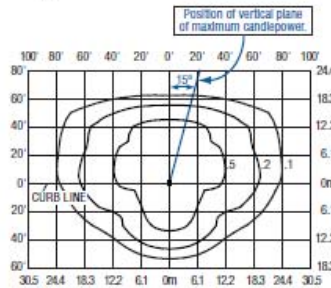
Isofootcandle plot of 6000K, 60 LED Type III Medium streetlight luminaire at 25' A.F.G. Luminaire with 6,831 initial delivered lumens operating at 525mA. Initial FC at grade.
