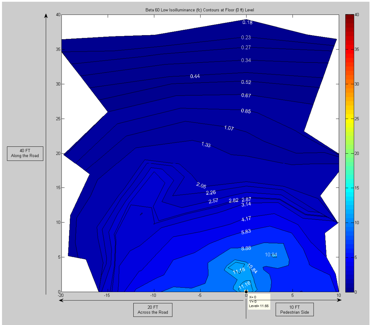
Figure 6: Contour Plot of Isoilluminance (fc) for Beta 60 LED Low Driver Setting at the Floor (0 Feet) Level on Measurement Grid
